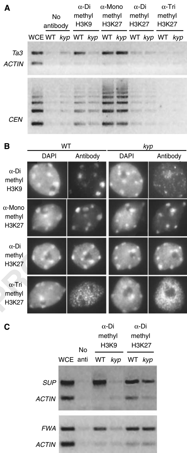
Figure 3 Colocalization of methyl H3K9 and H3K27 at heterochromatin. (A) ChIP analysis showing methyl H3K9 and H3K27 enrichment at the Ta3 retrotransposon and CEN repeats, relative to ACTIN . kyp affects levels of methyl H3K9 but not mono-, di-, or trimethyl H3K27. ACTIN is used for normalization, and the amount of chromatin used in each sample (for both the Ta3 and CEN experiments) was adjusted so that an equal amount of ACTIN was amplified. WCE, whole-cell extract. (B) Distribution of mono-, di-, and trimethyl H3K27 in interphase leaf nuclei. Mono- and dimethyl H3K27 are enriched at DAPI-stained chromocenters, while trimethyl H3K27 signals are more evenly distributed. kyp reduces dimethyl H3K9 at heterochromatin, but not H3K27 methylation. (C) ChIP analysis showing enrichment of both H3K9 and H3K27 methylation at SUPERMAN and FWA relative to ACTIN .
